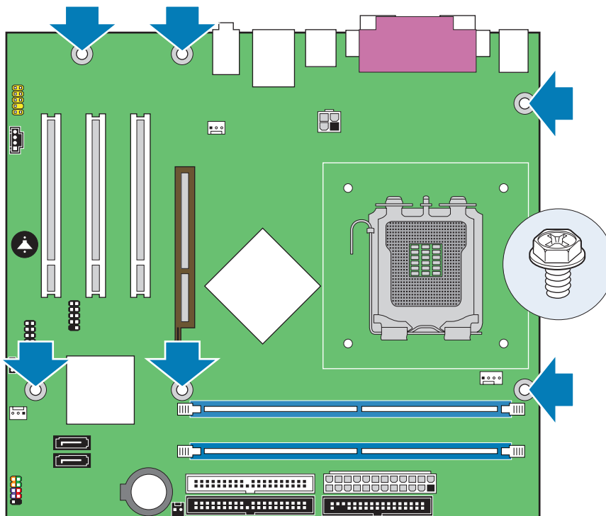
Figure 5. Desktop Board D865GSA Mounting Screw Hole Locations
